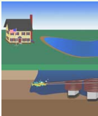
Pond Loop: coils of piping are submerged in a pond, slinky piping can also be used for this application.
